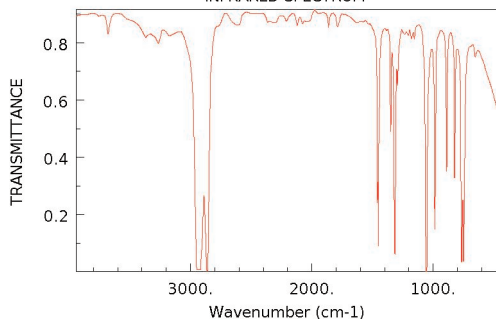
BICYCLO[2.2.2]OCTANE, 1,4-DIAZA- INFRARED SPECTRUM
