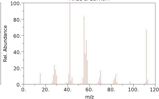
Triethylenediamine MASS SPECTRUM
